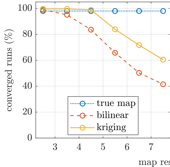
Threshold
